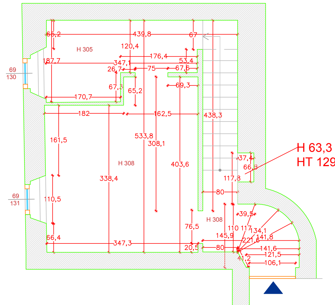
PIANO TERRA
